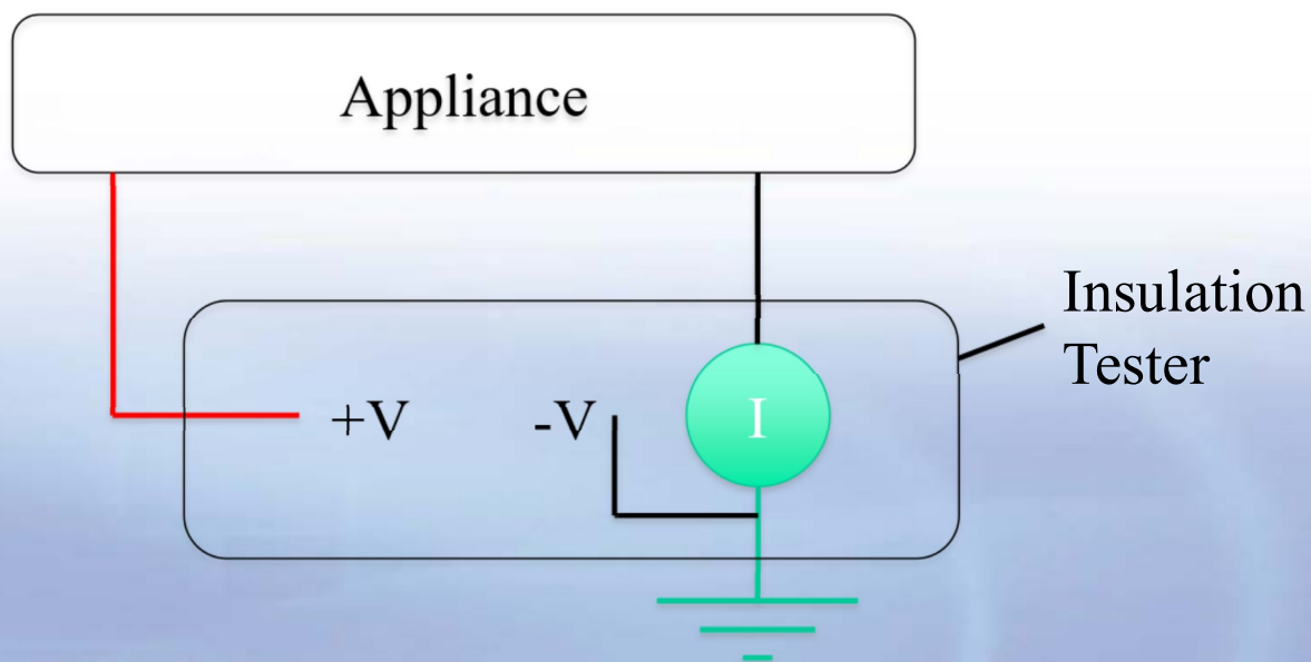
Basic Block Diagram of Insulation Tester
